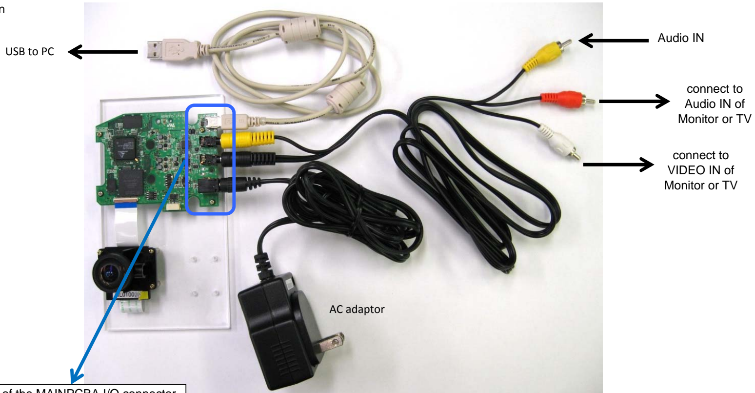
Detail of the MAINPCBA I/O connector
