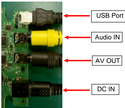
Detail of the MAINPCBA I/O connector
